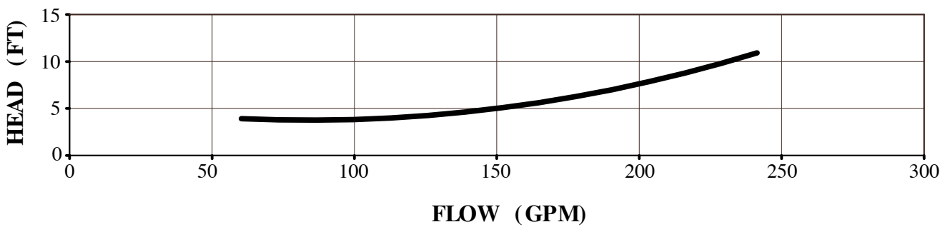
NPSHR (8" Impeller)
