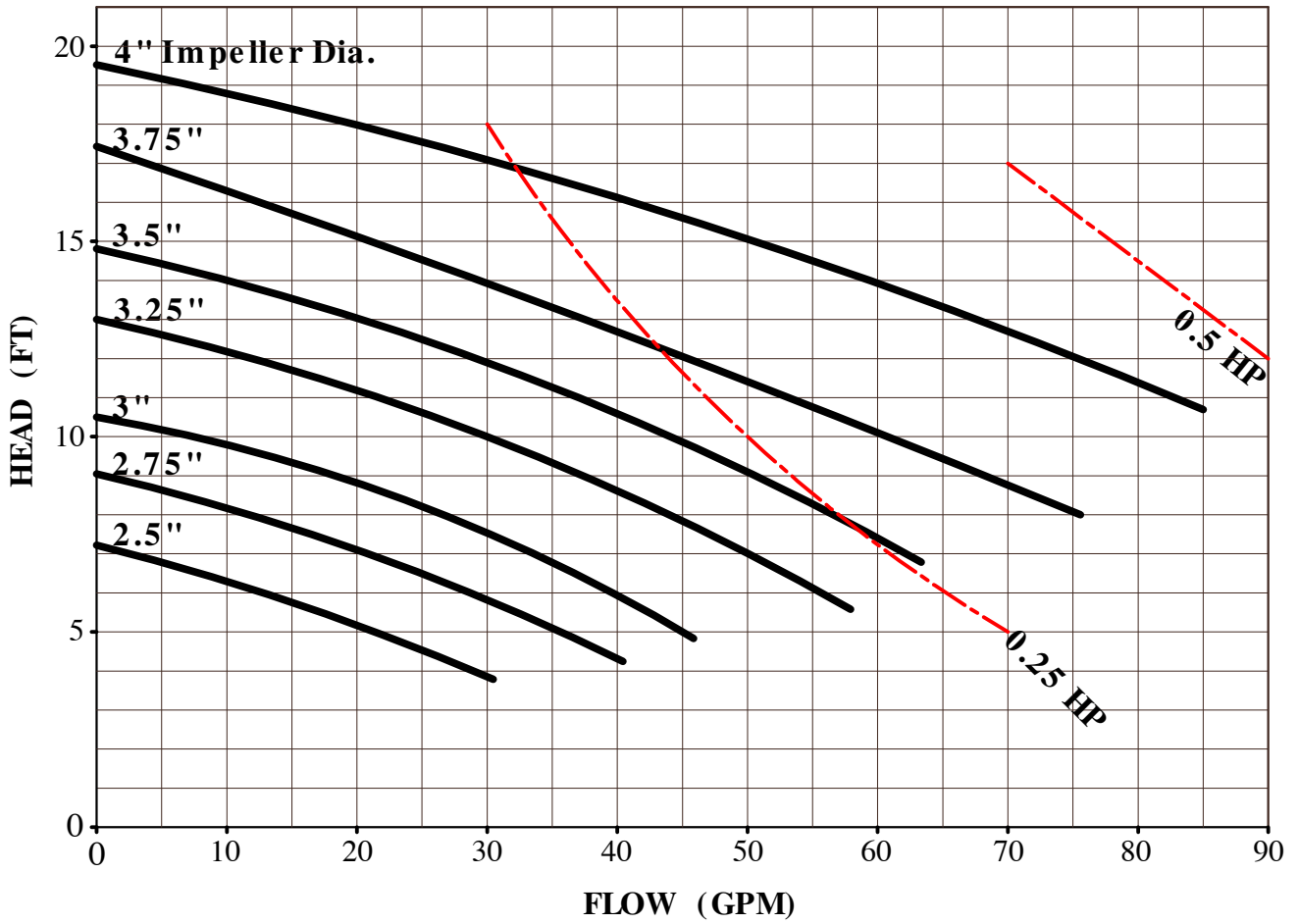
C214 @ 1750 RPM
