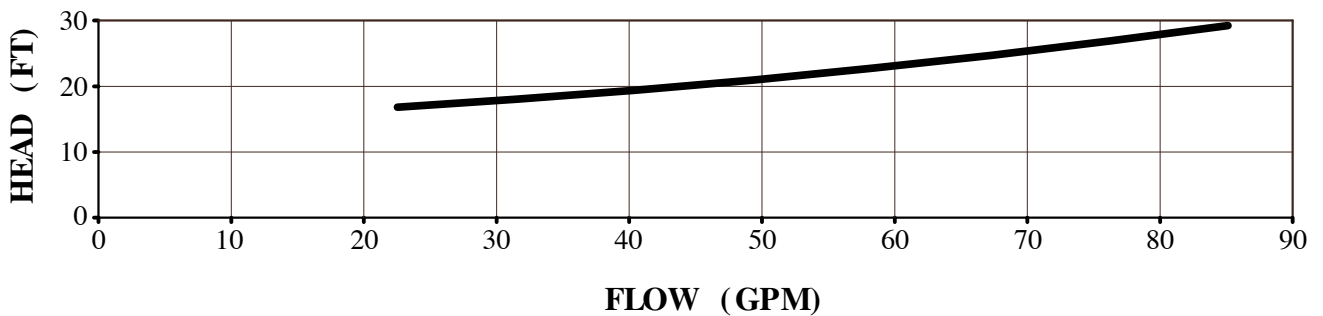
NPSHR (4" Impeller)
