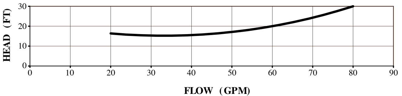
NPSHR (4" Impeller)
