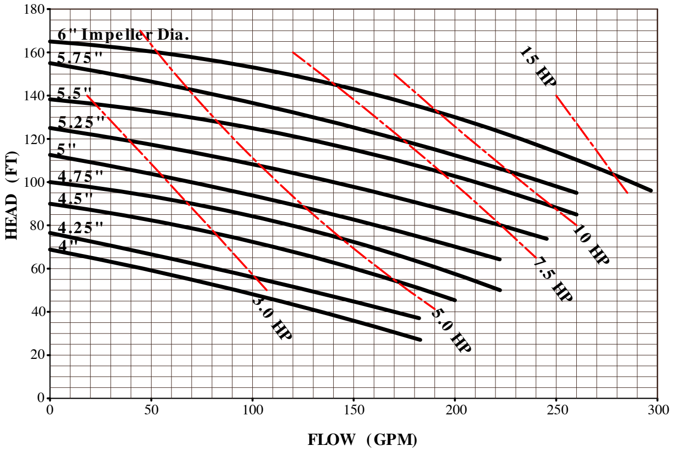
C216 @ 3500 RPM
